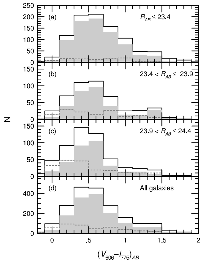
FIG. 9.— Histogram showing the number of galaxies placed on masks ( solid black line ) and number of redshifts measured ( grey histogram ), as a function of the V_{606} - i_{775} color. Also shown is the distribution of failed redshift measurements ( dashed line ). Panels (a) through (c) show the color distributions for different magnitude ranges, and panel (d) shows the distribution for the entire sample. While the color distributions of galaxies placed on masks and of those successfully observed do not change significantly with magnitude, the color distribution of redshift failures shows a clear trend of becoming bluer at fainter apparent magnitude.
